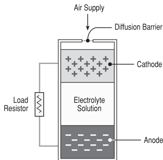
Construction of Galvanic Cell
