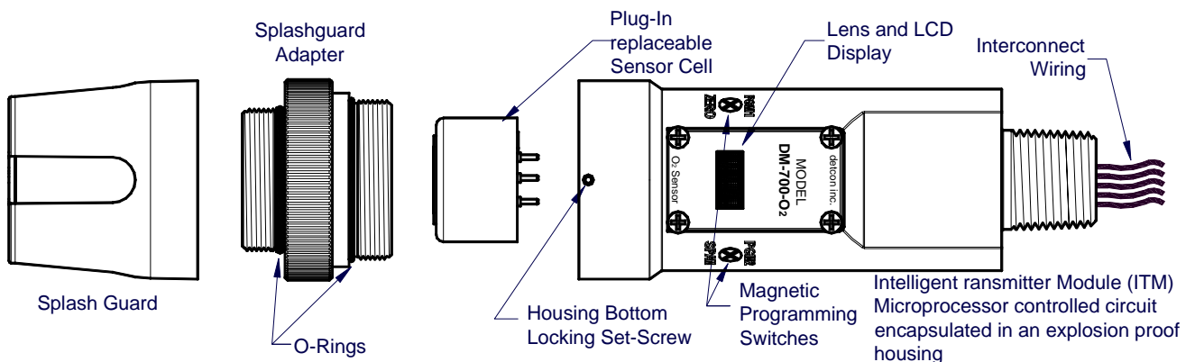
Figure 5 Sensor Assembly Breakaway
