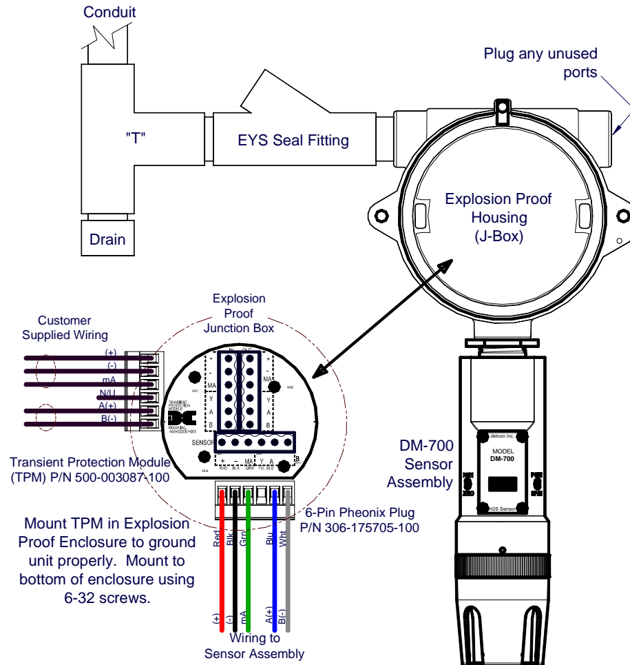
Figure 9 Typical Installation
