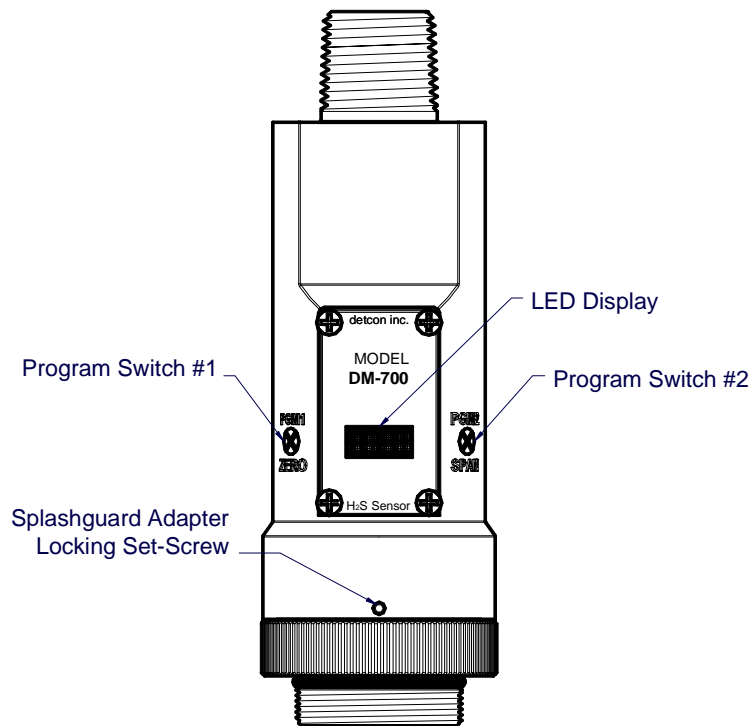
Figure 4 Sensor Assembly Front View
