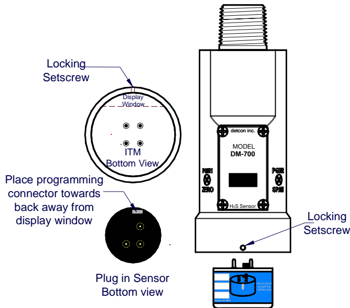
Figure 16 Sensor Cell and ITM Mating
