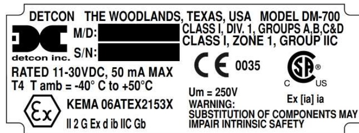
Figure 7 ATEX Approval Label
