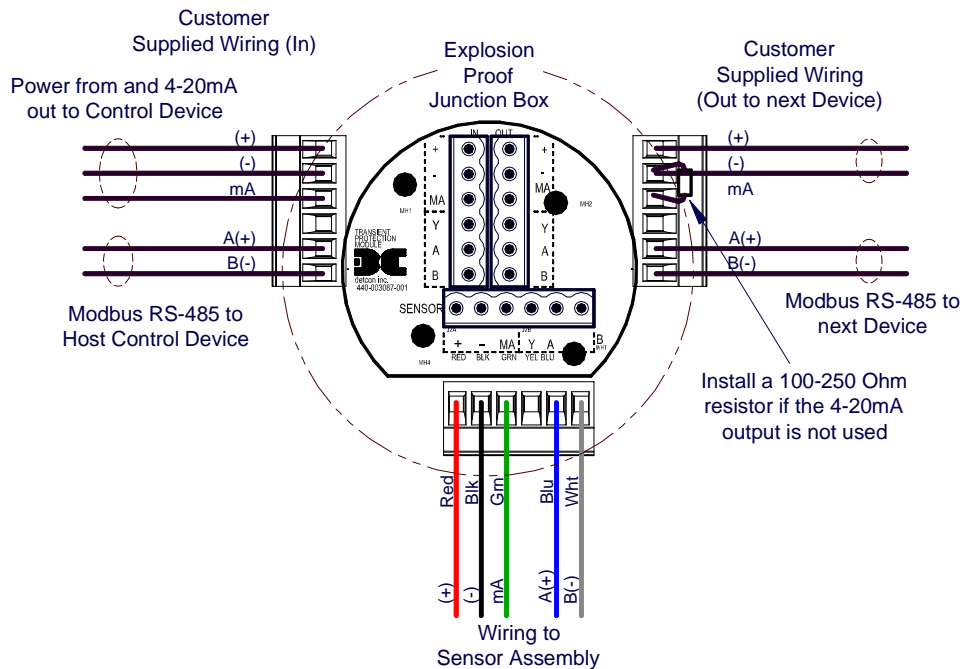
Figure 10 Sensor Wire Connections
