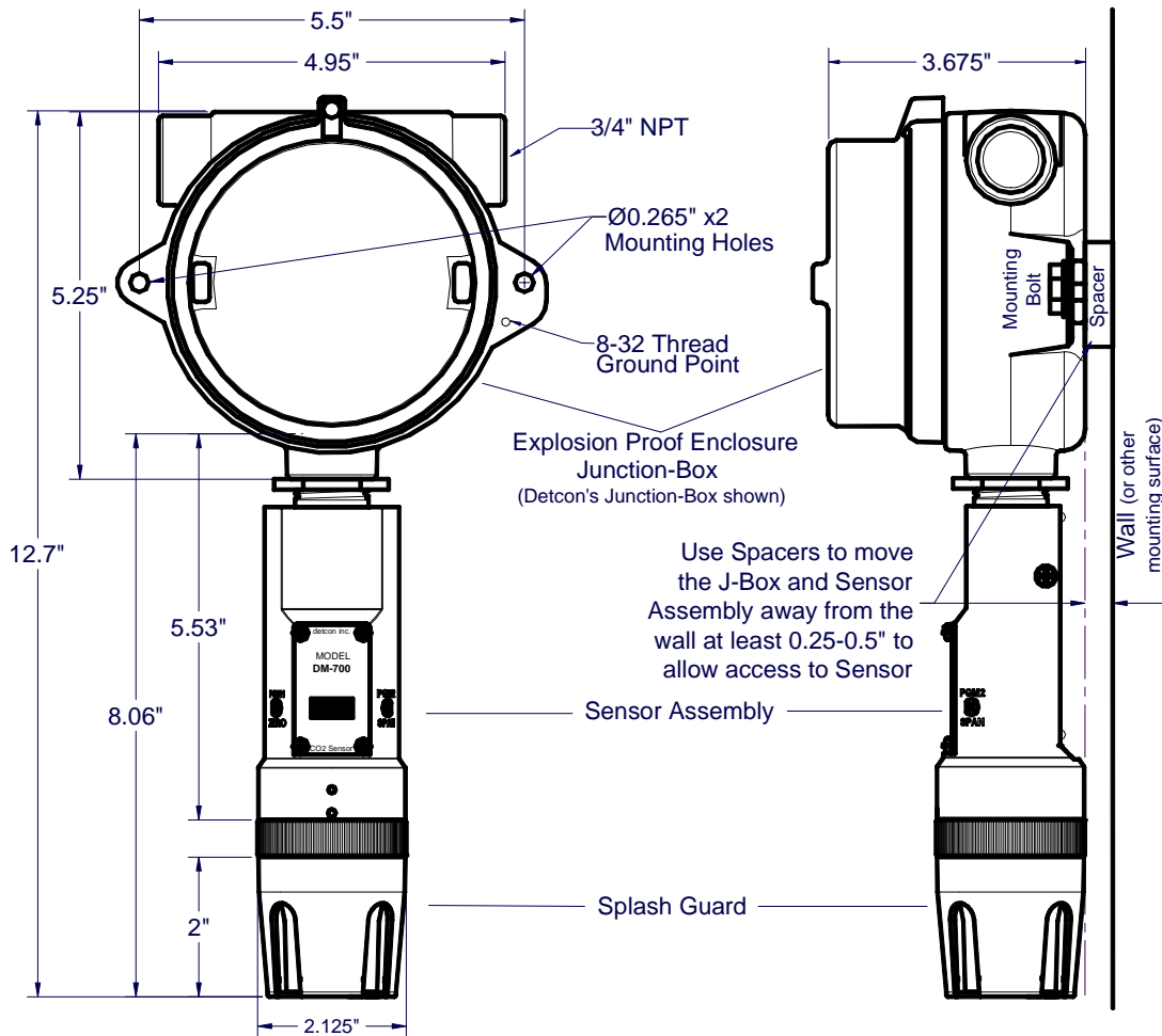
Figure 8 Outline and Mounting Dimensions
