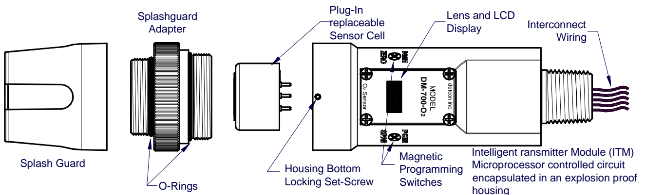
Figure 14 Sensor Assembly
