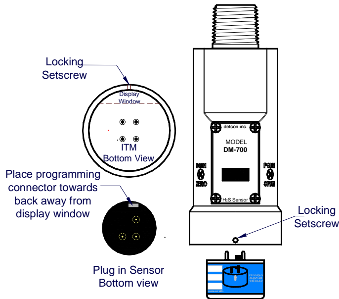
Figure 15 Sensor Cell and ITM Mating
