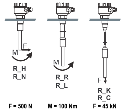
Figure 1. Maximum allowed torque and force
