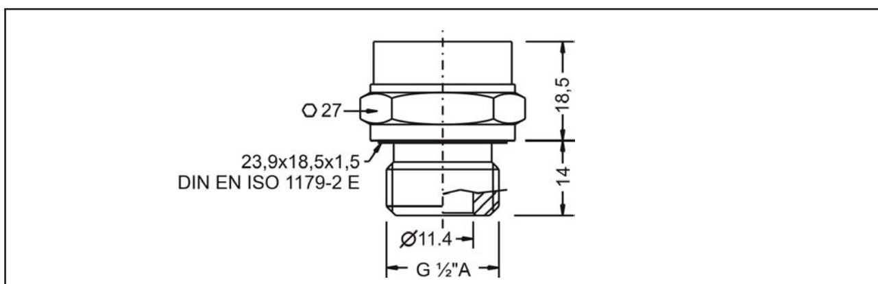
Type 2 – Thread ISO 228-1 – G \frac{1}{2} " A, DIN EN ISO 1179-2 E, inner bore
