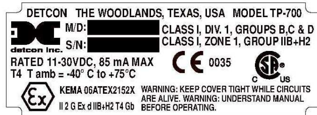
Figure 5 ATEX Approval Label
