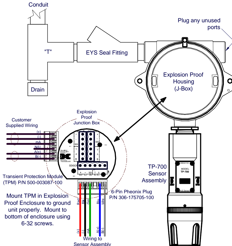
Figure 7 Typical Installation
