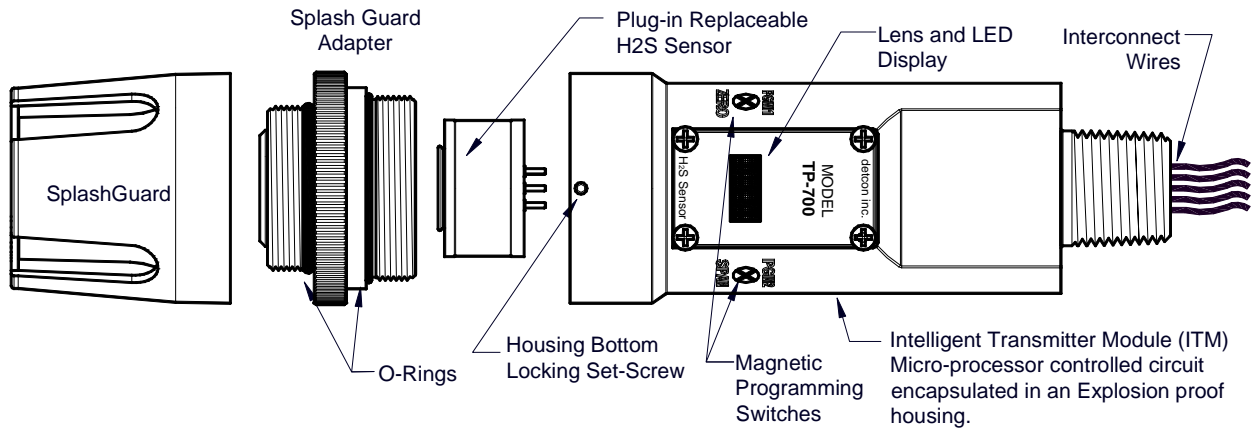
Figure 3 Sensor Assembly Breakaway
