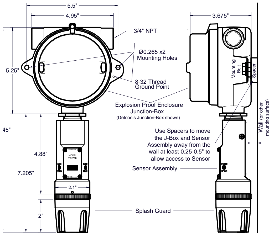
Figure 6 Outline and Mounting Dimensions
