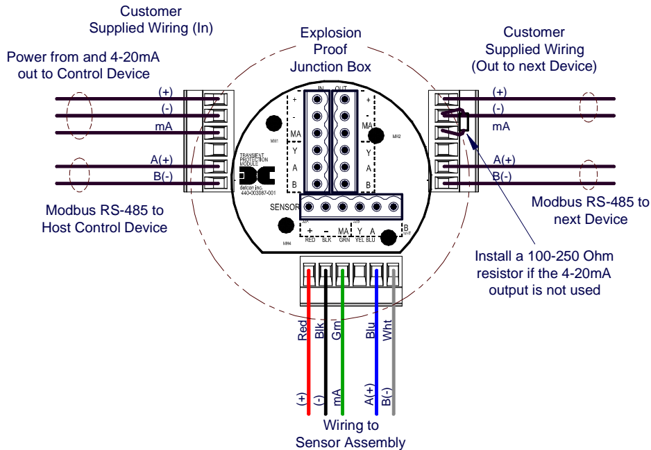
Figure 8 Sensor Wire Connections
