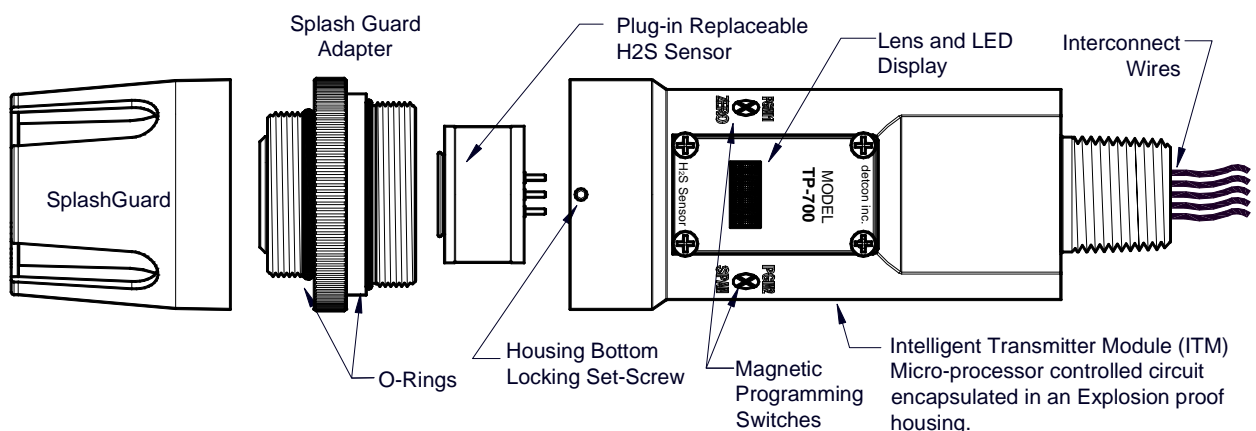
Figure 12 Sensor Assembly
